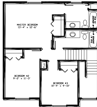
2nd Floor
