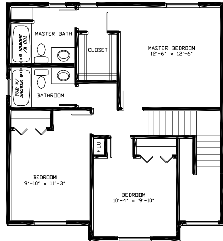
2nd Floor
