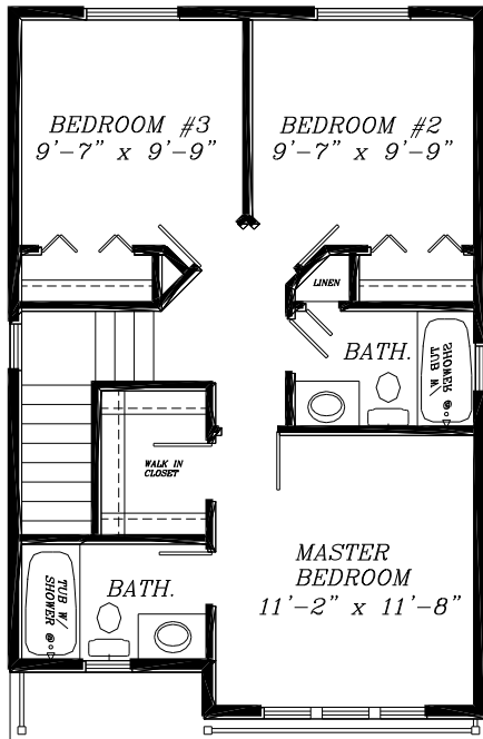
2nd Level
