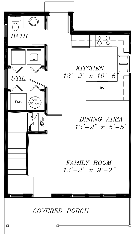
Floor Plan
