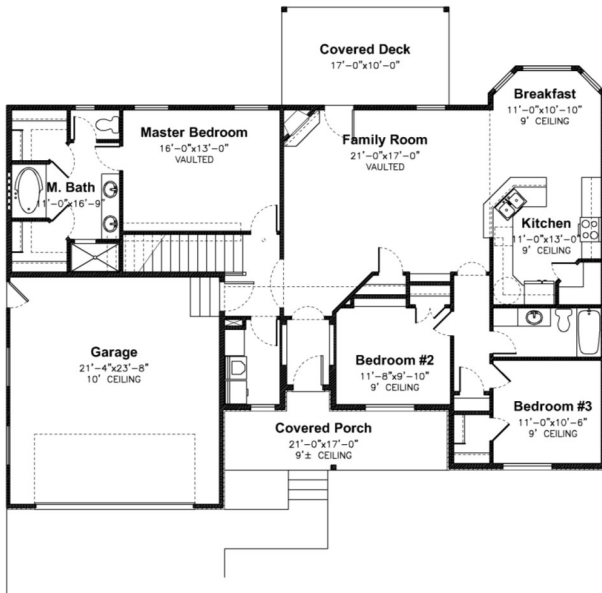
Main Floor
