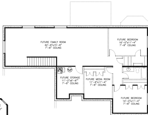
Basement Floor
