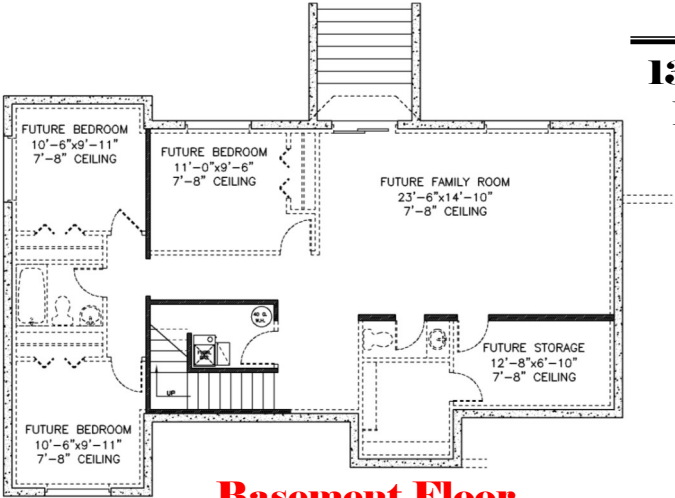
Basement Floor
