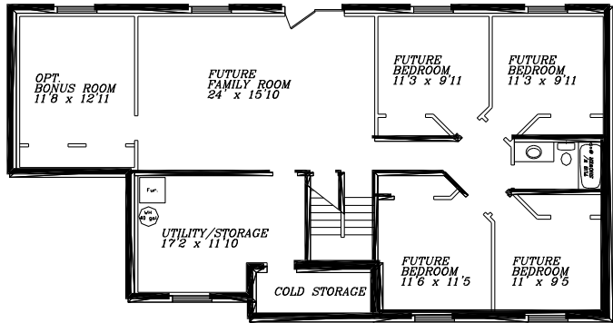
Basement
