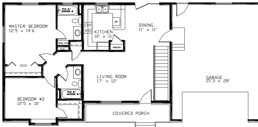
Floor Plan
