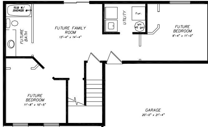
Basement
